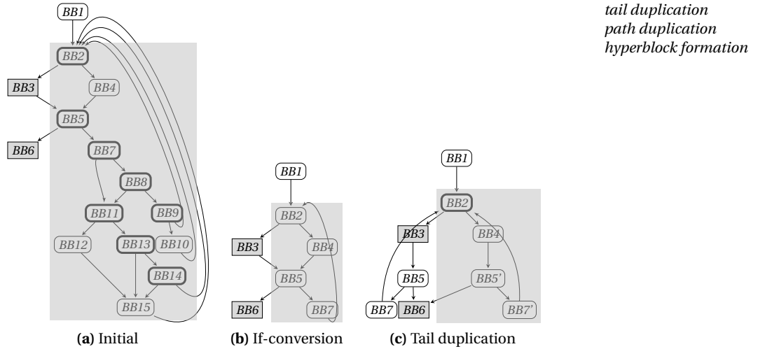
Fig. 18.11 If-conversion of wc (word count program). Basic blocks in the gray region cannot be if-converted. Tail duplication can be used to exclude BB3 from the to-be-if-converted region.
