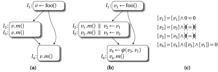
Fig. 12.4 Null pointer analysis as an example of forward data-flow analysis that takes information from the definitions and uses of variables (0 represents the fact that the pointer is possibly null, \emptyset if it cannot be).
