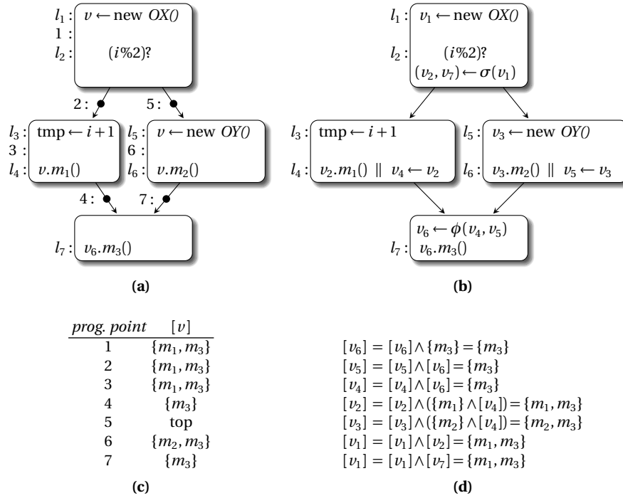
Fig. 12.3 Class inference analysis as an example of backward data-flow analysis that takes information from the uses of variables.
