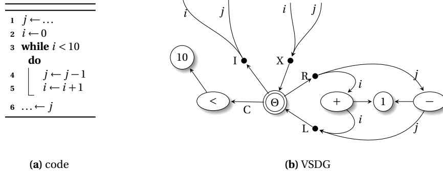
Fig. 13.7 An example showing a for loop. Evaluating X triggers it to evaluate the I value (outputting the value L ). While C evaluates to true, it evaluates the R value (which in this case also uses the \theta -node's L value). When C is false, it returns the final internal value through X . As i is not used after the loop there is no dependency on i at X .
