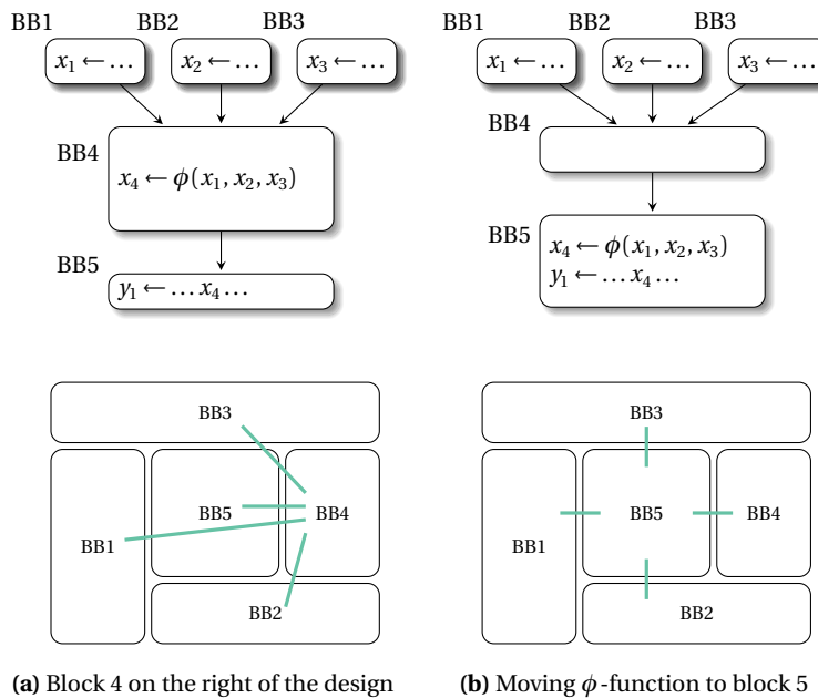
Fig. 20.8 Example of the impact of \phi -function movement in reducing hardware wire length
