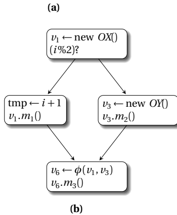
Fig. 12.10 (a) implementing \sigma -functions via single arity \phi -functions; (b) getting rid of copies and \sigma -functions.
