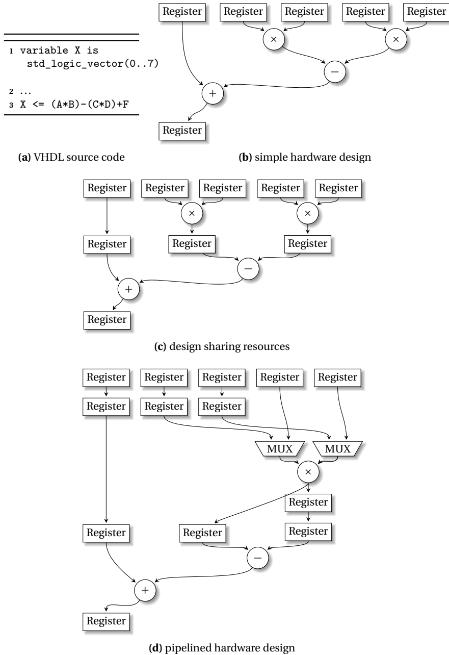
Fig. 20.1 Different variants of mapping a computation to hardware
