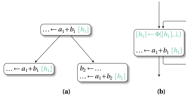
Fig. 10.4 Examples of expression renaming
