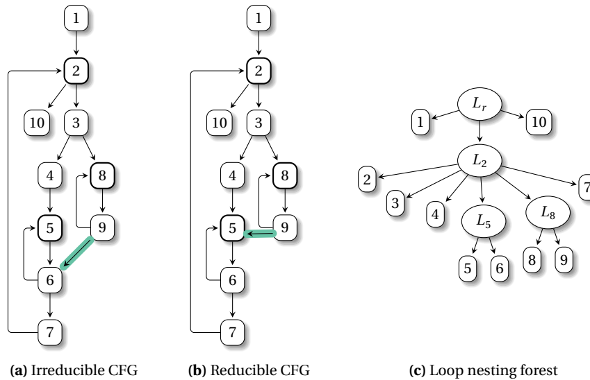
Fig. 8.3 A reducible CFG derived from an irreducible CFG, using the loop nesting forest. The transformation redirects edges arriving inside a loop to the loop header (here 9 \rightarrow 6 into 9 \rightarrow 5 ).
