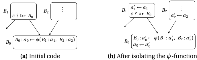
Fig. 19.1 Isolation of a \phi -node*
