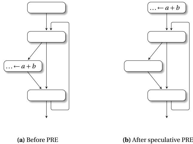
Fig. 10.6 Speculative loop-invariant code motion
