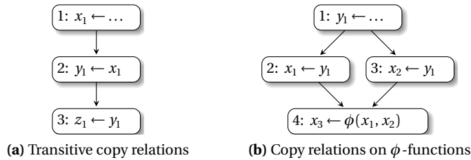
Fig. 7.3 Analysis of copy-related variables
