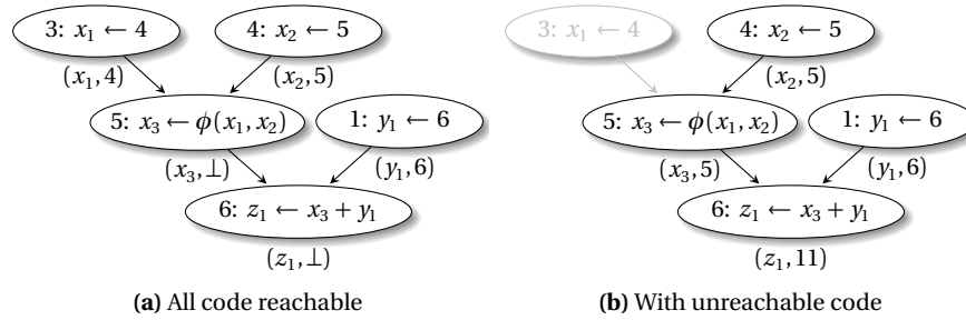
Fig. 7.2 Sparse conditional data-flow propagation using SSA graphs
