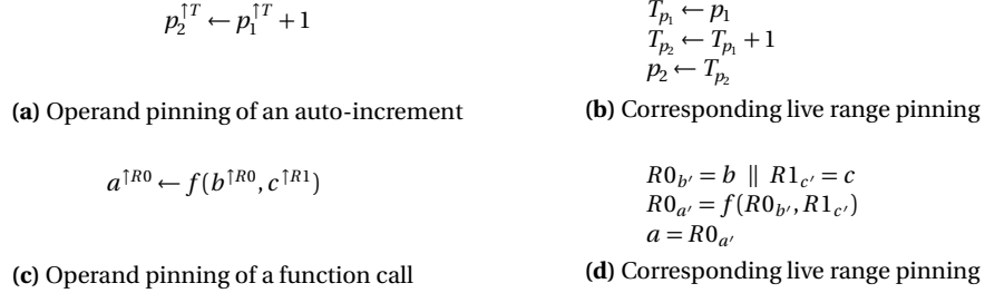
Fig. 19.4 Operand pinning and corresponding live range pinning
