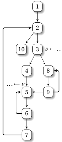
Fig. 8.1 An example of a reducible CFG. Forward CFG is represented using full edges; back-edges are thickened. Backward pass on forward CFG sets v as live-in of node 5, but not of node 2. Forward pass on loop nesting forest then sets v as live at node 6 but not at node 7.
