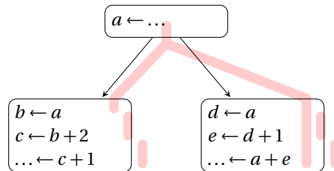
Fig. 19.6 Variables live ranges are sub-trees of the dominator tree*
