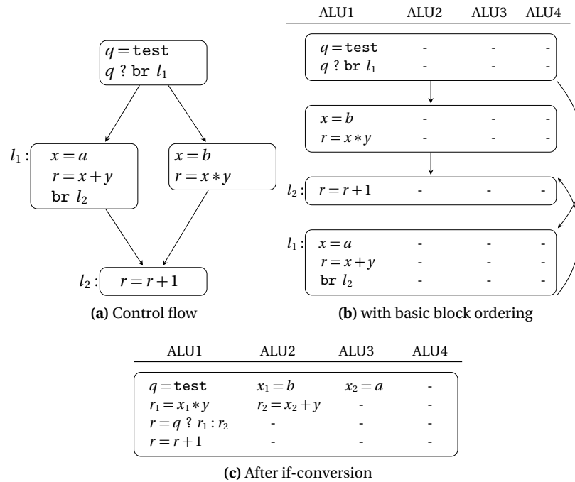
Fig. 18.1 Static schedule of a simple region on a 4-issue processor.
