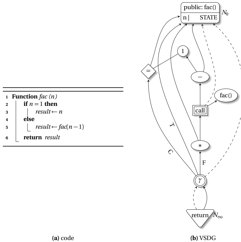
Fig. 13.5 A recursive factorial function, whose VSDG illustrates the key graph components—value dependency edges (solid lines), state dependency edges (dashed lines), a const node, a call node, a \gamma -node, a conditional node, and the function entry and exit nodes.
