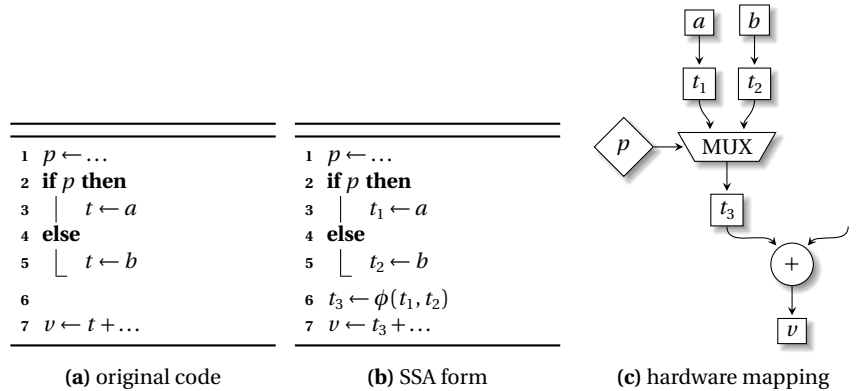
Fig. 20.2 Basic hardware mapping using SSA representation
