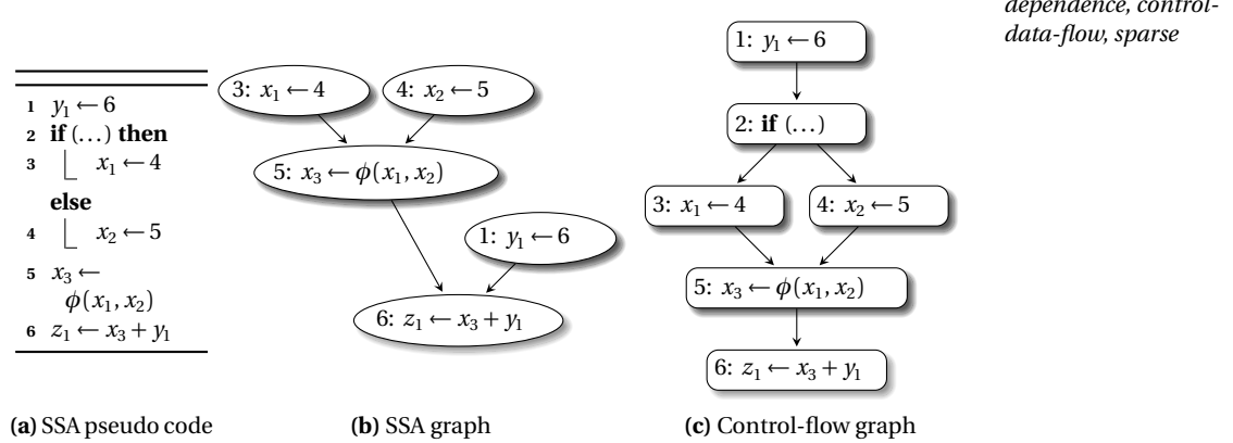
Fig. 7.1 Example program and its SSA graph
