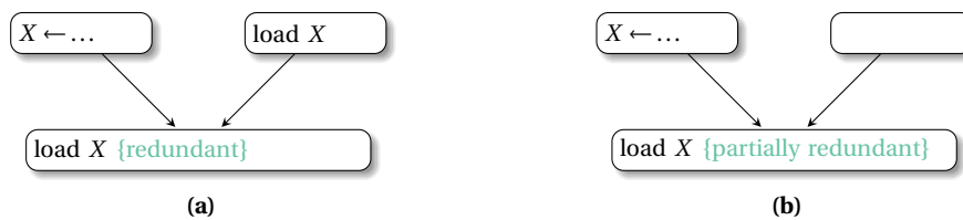
Fig. 10.9 Redundant loads after stores
