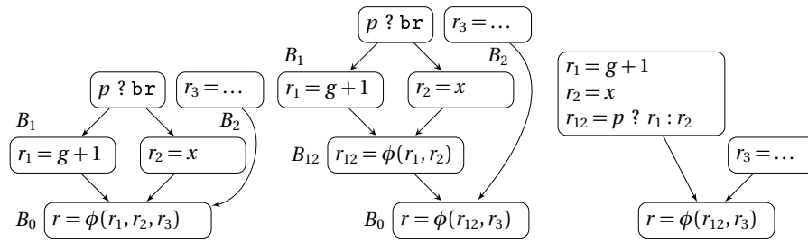
Fig. 18.5 \phi reduction
