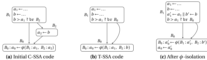
Fig. 19.3 Copy-folding followed by empty block elimination can lead to SSA code for which destruction is not possible through simple copy insertion
