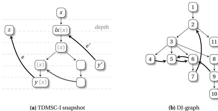
Fig. 4.4 (a) Snapshot during execution of the TDMSC-I algorithm and (b) Recall of running example.
