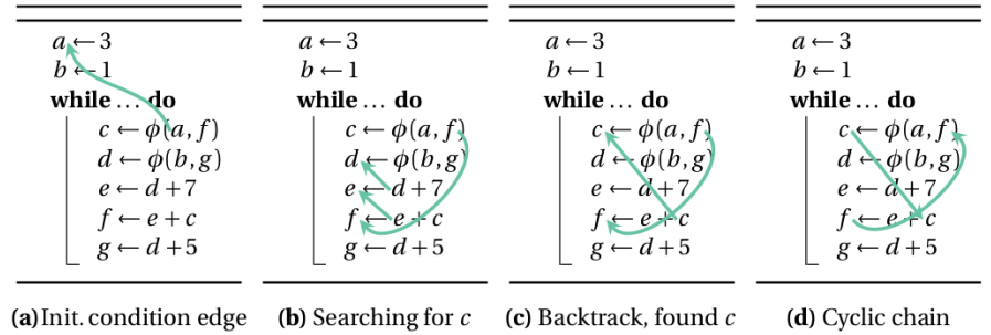
Fig. 9.1 Detection of the cyclic definition using a depth first search traversal of the use-def chains.
