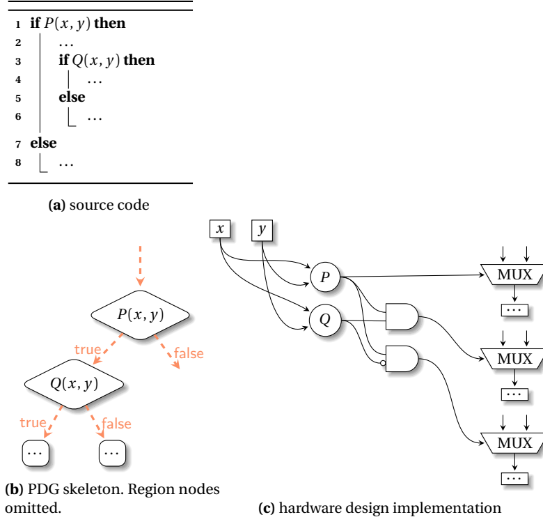
Fig. 20.6 Use of the predicates in region nodes of the PDG for mapping into the multiplexers associated with each \phi -function
