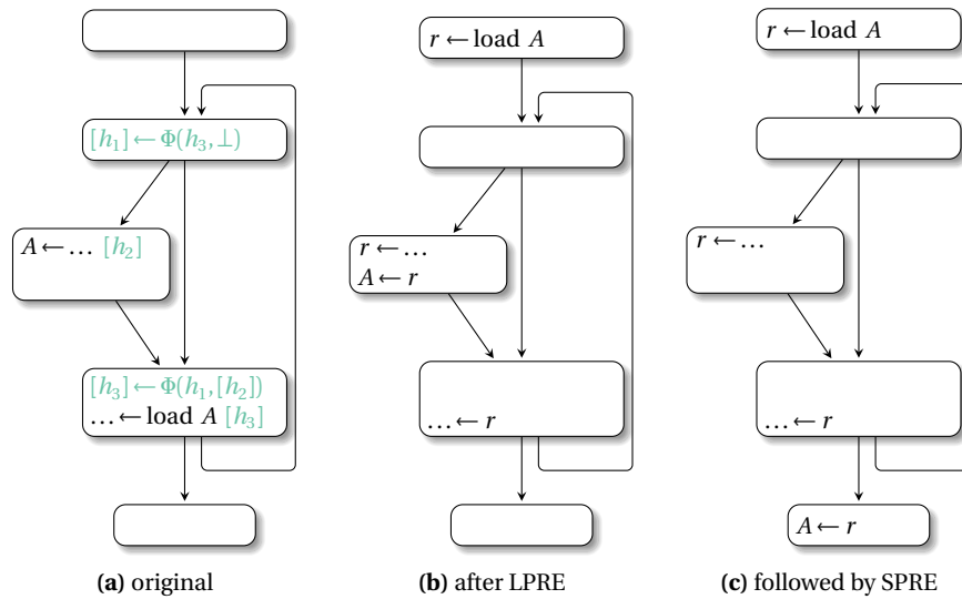
Fig. 10.10 Register promotion via load PRE followed by store PRE
