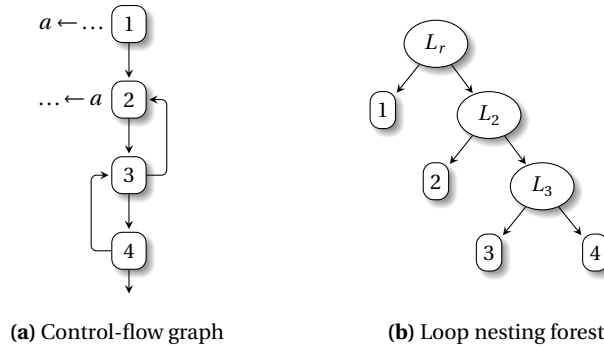
Fig. 8.2 Bad case for iterative data-flow analysis.
