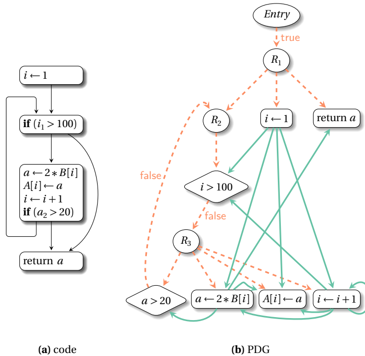
Fig. 13.2 Example code translated into a PDG. Dashed/full edges respectively represent control/data dependencies.
