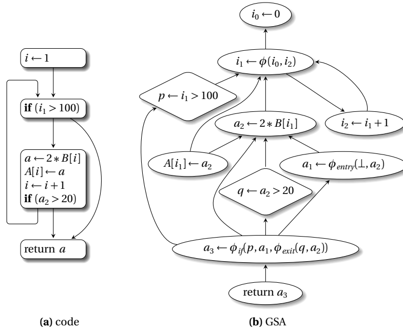
Fig. 13.3 A graph representation of our sample code in (demand-based) GSA form.
