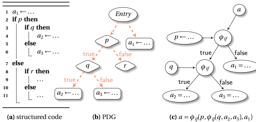
Fig. 13.4 (a) A structured code; (b) the PDG (with region nodes ommited); (c) the DAG representation of the nested gated \phi_{if}
