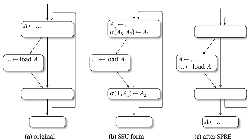
Fig. 10.11 Example of program in SSU form and the result of applying SSUPRE
