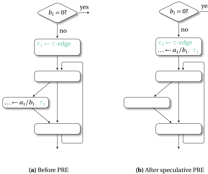
Fig. 10.7 Speculative and fault-safe loop-invariant code motion
