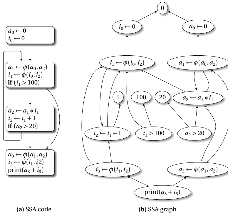
Fig. 13.1 Some SSA code translated into an SSA graph. Note how edges demand the input values for a node.
