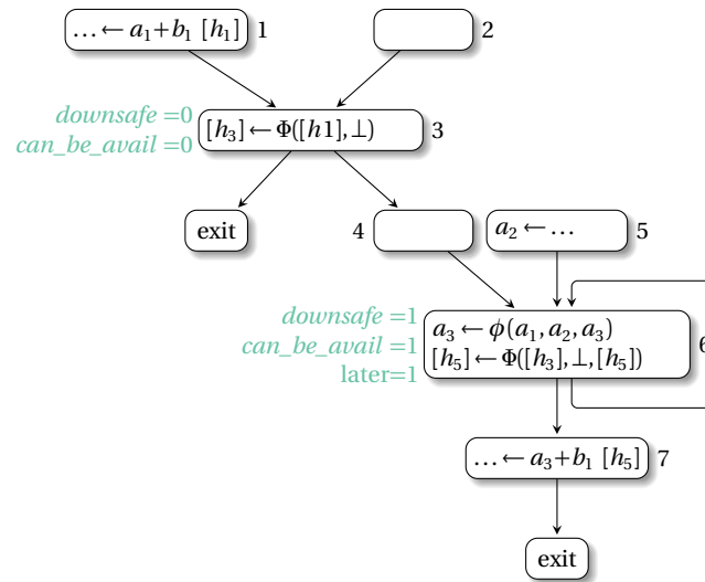
Fig. 10.5 Example to show the need of the later attribute
