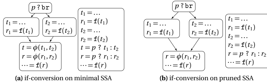
Fig. 18.8 SSA predicate minimality
