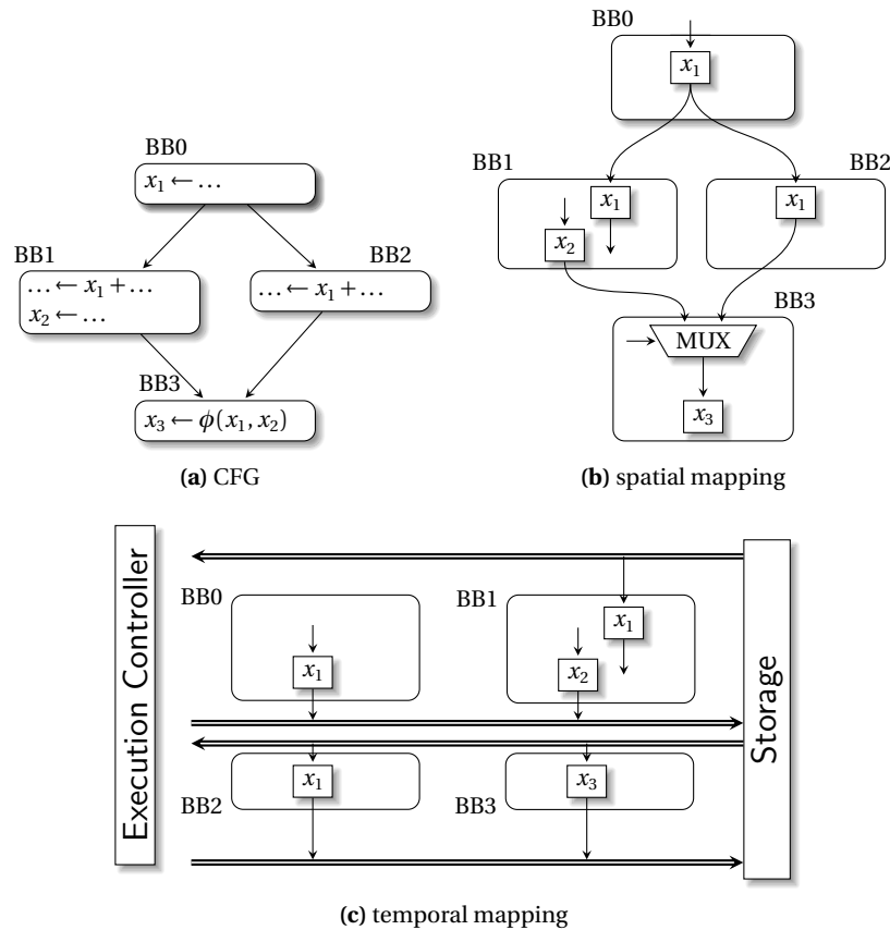
Fig. 20.3 Combination of hardware circuits for multiple basic blocks
