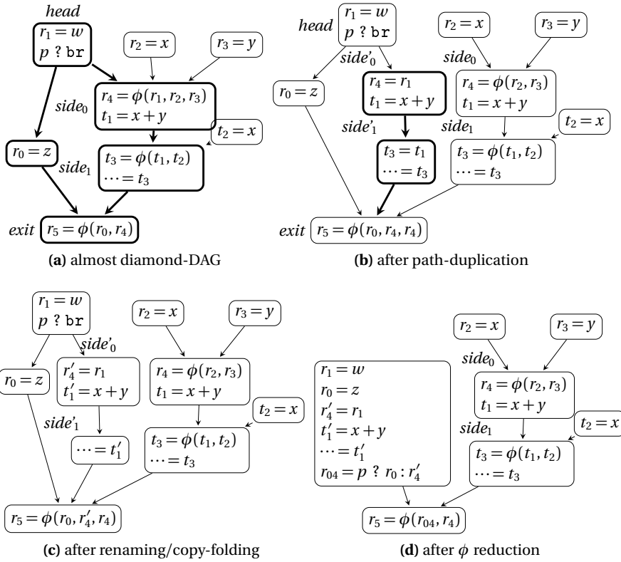
Fig. 18.6 Path duplication
