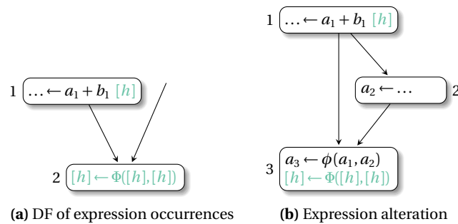
Fig. 10.3 Examples of \Phi insertion
