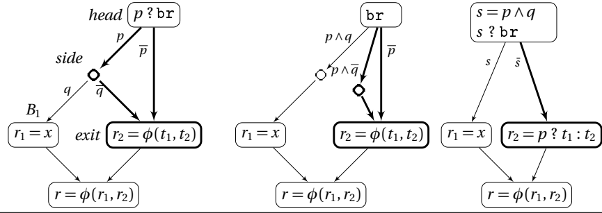
Fig. 18.7 convergent conjunctive merge
