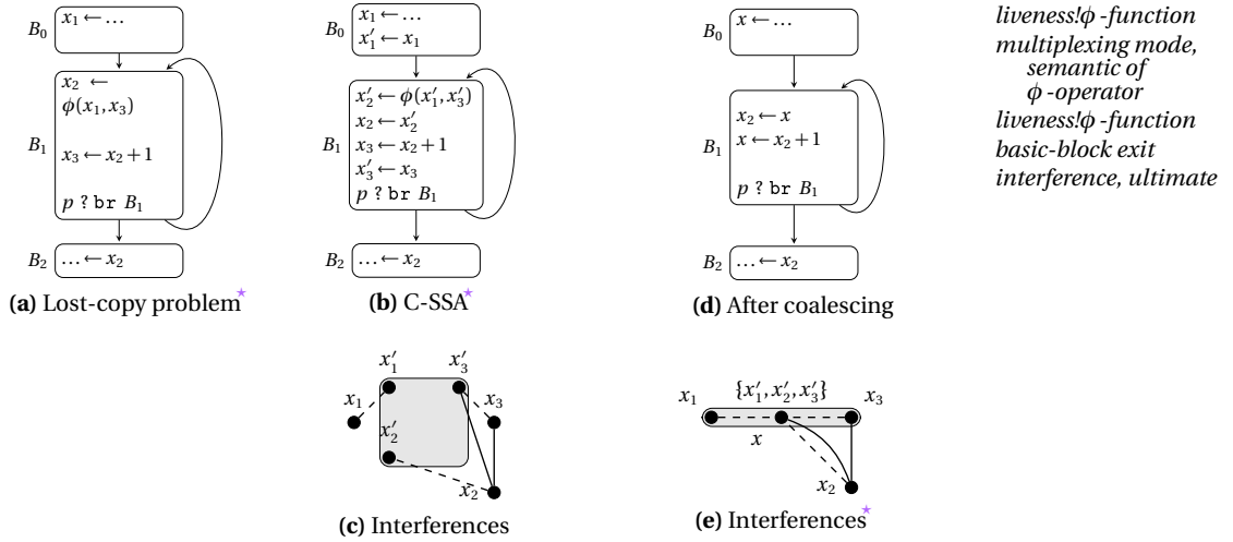
Fig. 19.5 SSA destruction for the lost-copy problem.
