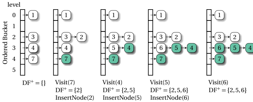
Fig. 4.3 Phases of Algorithm 4.1 for S = \text{Defs}(v) = \{1, 3, 4, 7\} .
