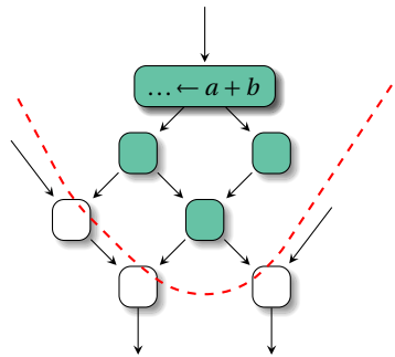
Fig. 10.2 Dominance frontiers (dashed) are boundaries between fully (highlighted basic blocks) and partially redundant regions (normal basic blocks).
