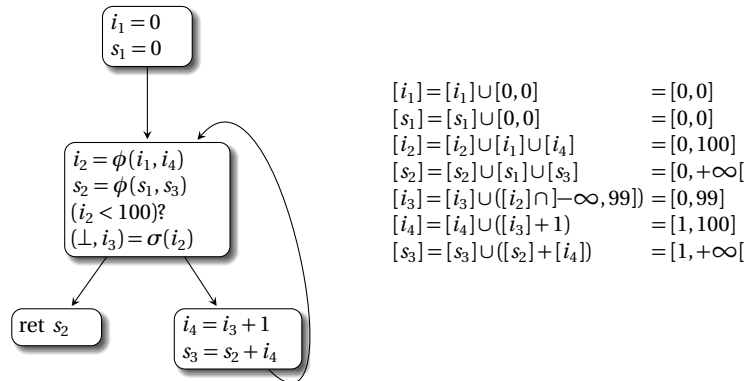
Fig. 12.2 Live-range splitting on Figure 12.1 and a solution to this instance of the range analysis problem.
