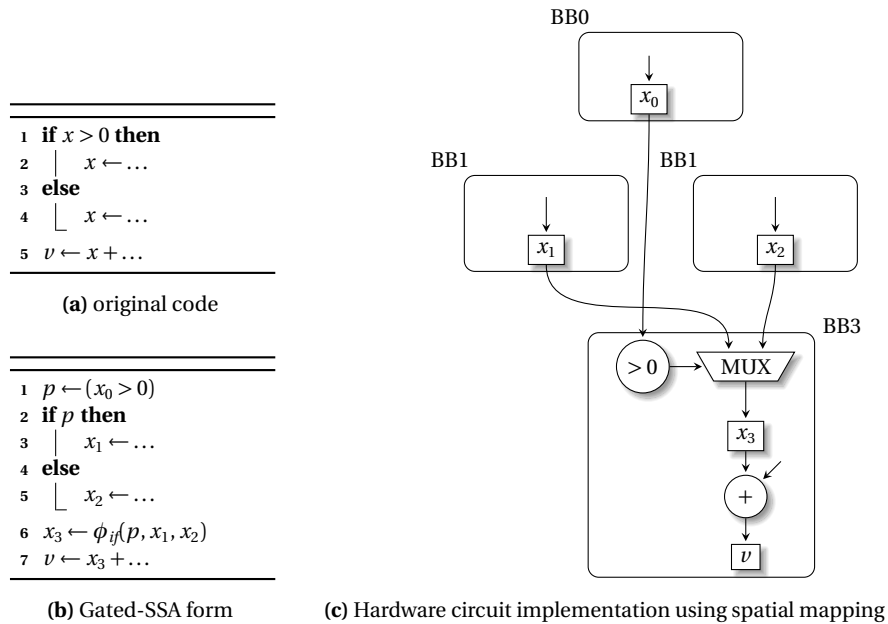
Fig. 20.5 Hardware generation example using Gated-SSA form
