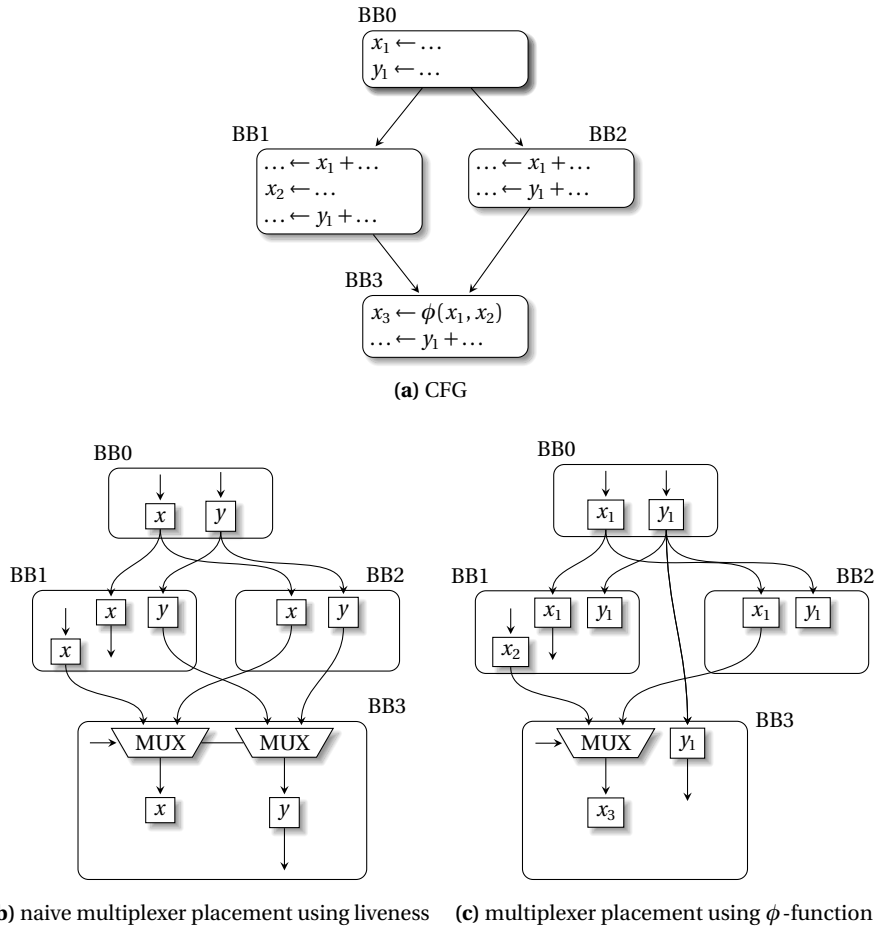
Fig. 20.4 Mapping of variable values across hardware circuit using spatial mapping
