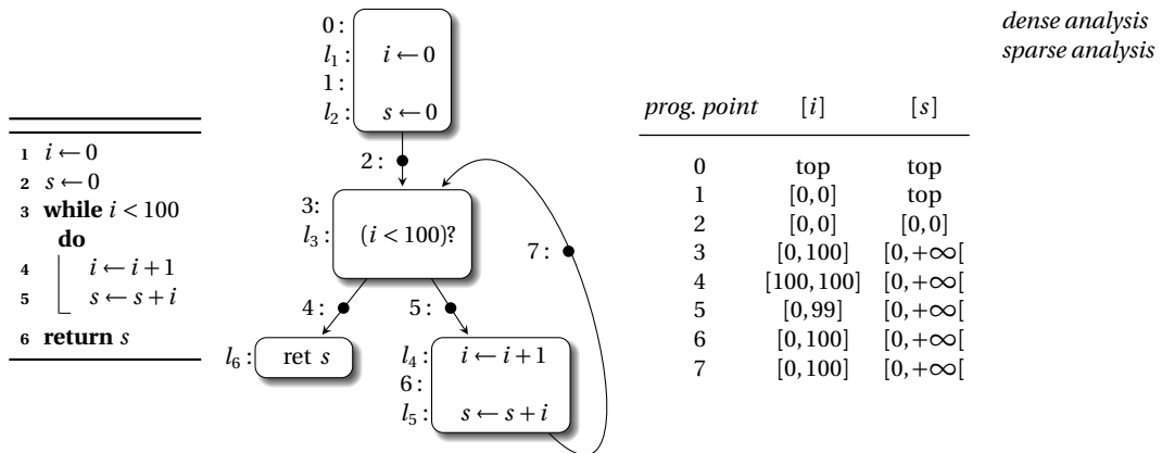
Fig. 12.1 An example of a dense data-flow analysis that finds the range of possible values associated with each variable at each program point.
