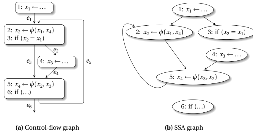
Fig. 7.4 \phi -functions in loops often obfuscate copy relations.
