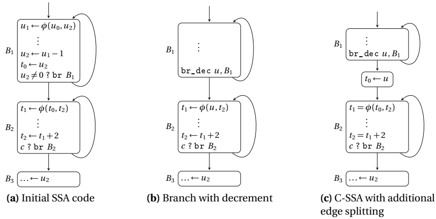
Fig. 19.2 Copy insertion may not be sufficient. \text{br\_dec } u, B_1 decrements u , then branches to B_1 if u \neq 0 .
