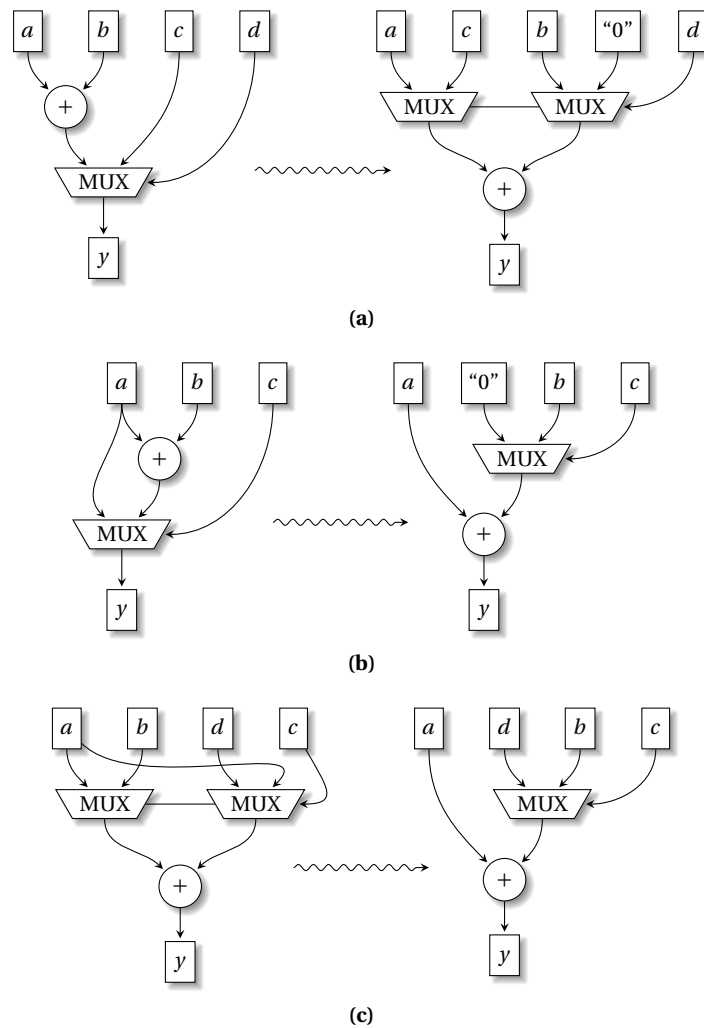
Fig. 20.7 Multiplexer-Operator transformations: juxtaposition of a multiplexer and an adder (a,b); reducing the number of multiplexers placed on the input of an adder (c)
